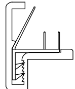
NOR510 Holder complete with NOR515 Seal
