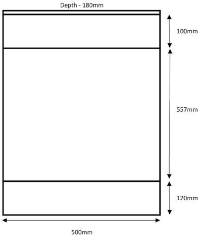
500mm WC UNIT
