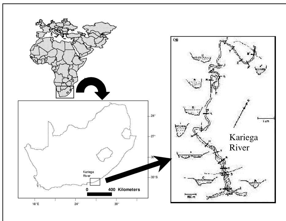
Figure 2.18. Location and morphometry of the Kariega River.
