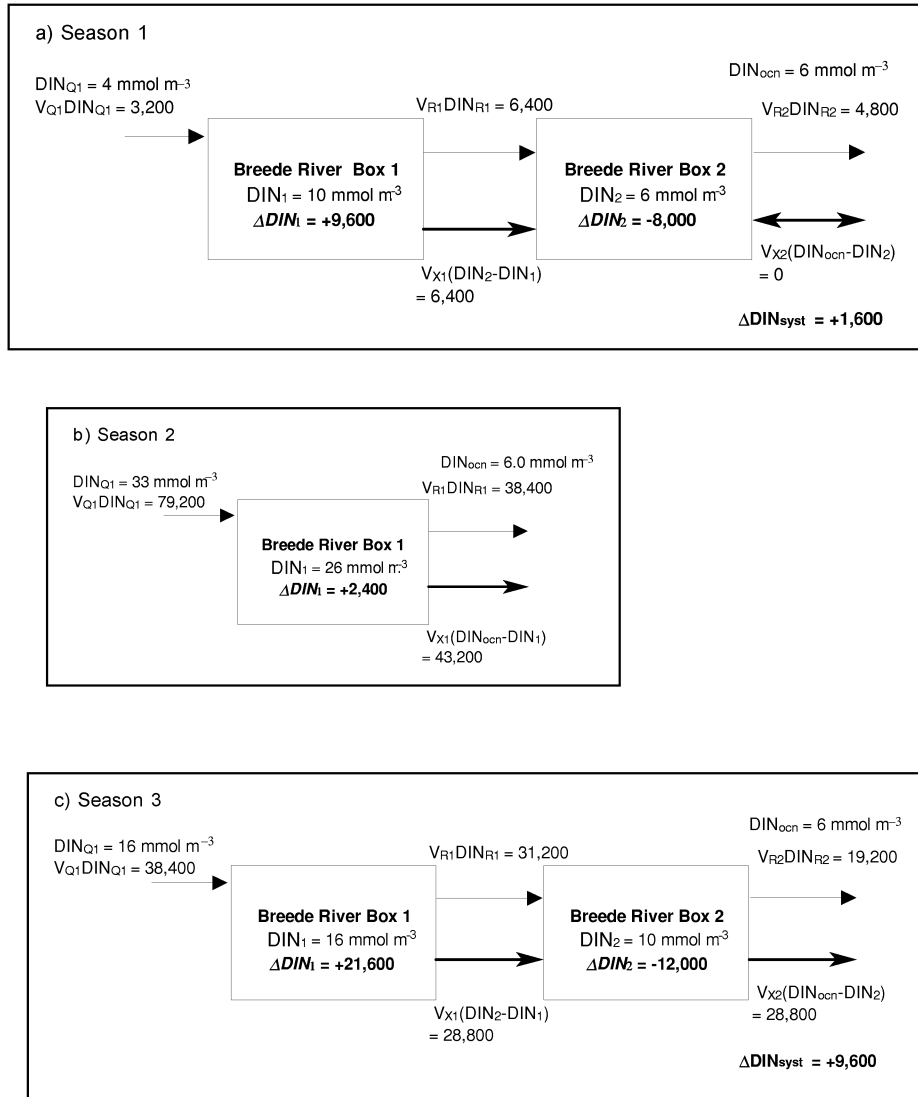
Figure 2.12. DIN budgets for the Breede River system in Season 1 (a), season 2 (b) and Season 3 (c). Flux in \text{mol day}^{-1} .
