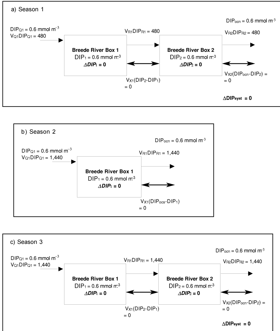
Figure 2.11. DIP budgets for the Breede River system in Season 1 (a), season 2 (b) and Season 3 (c). Flux in \text{mol day}^{-1} .
