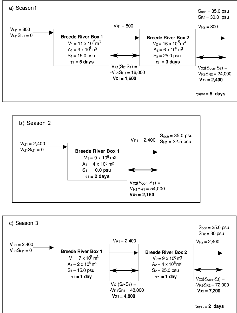
Figure 2.10. Water and salt budgets for the Breede River system in Season 1 (a), Season 2 (b) and Season 3 (c). Water flux in 10^3 \text{ m}^3 \text{ day}^{-1} and salt flux in 10^3 \text{ psu-m}^3 \text{ day}^{-1} .
