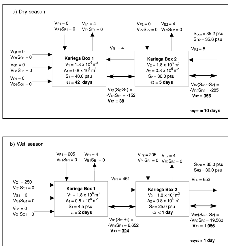
Figure 2 19. Water and salt budgets for Kariega River estuary in the dry (a) and wet (b) periods. Water flux in 10^3 \text{ m}^3 \text{ day}^{-1} and salt flux in 10^3 \text{ psu-m}^3 \text{ day}^{-1} .
