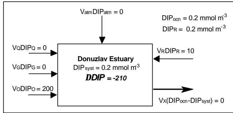
Figure 3.12. DIP budget for the Donuzlav estuary. Flux in \text{mol d}^{-1} .
