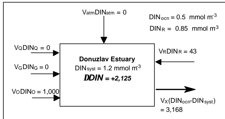
Figure 3.13. DIN budget for the Donuzlav estuary. Flux in \text{mol d}^{-1} .
