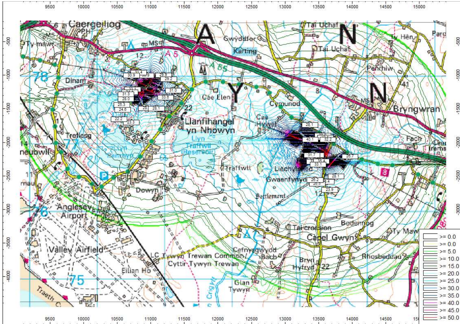
NOISE MAP 8-1: NOISE CONTOURS OF SOLAR FARM
