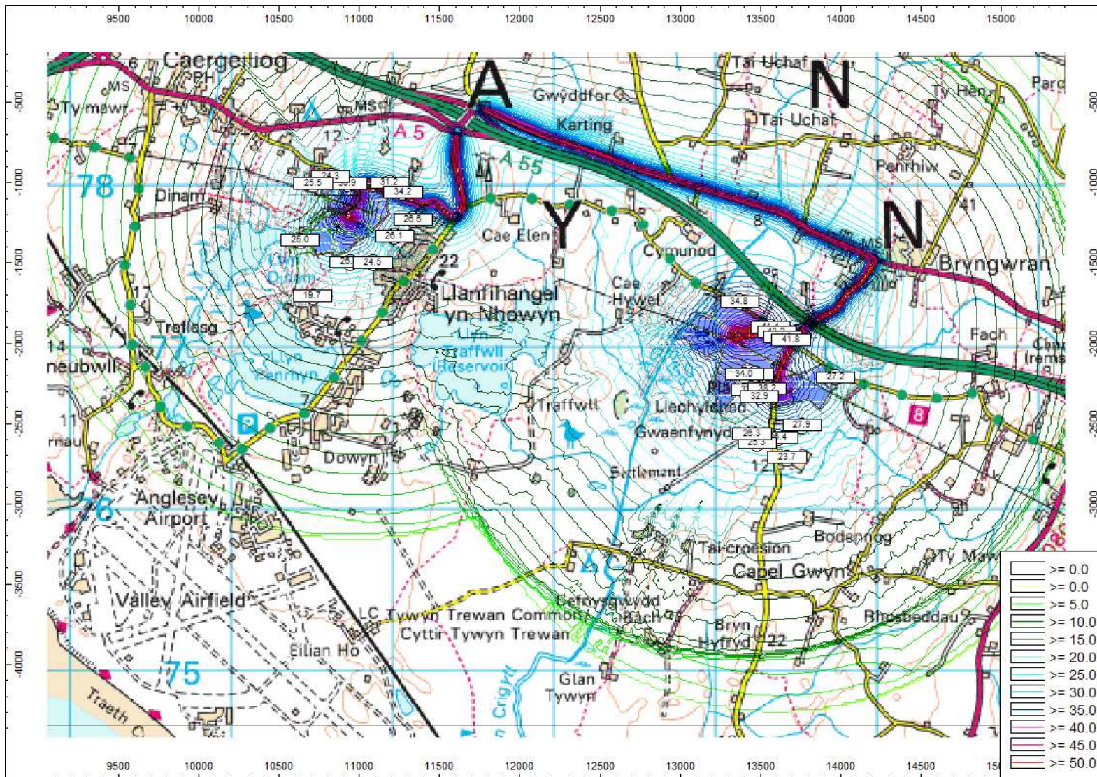
NOISE MAP 8-2: NOISE CONTOURS OF CONSTRUCTION ROAD TRAFFIC
